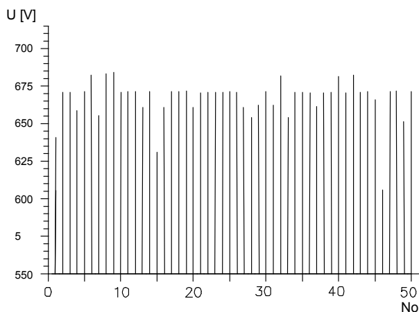
Fig. 10(b). Chronological series of measured values of GFS d.c. Breakdown Voltage immediately after radiation
