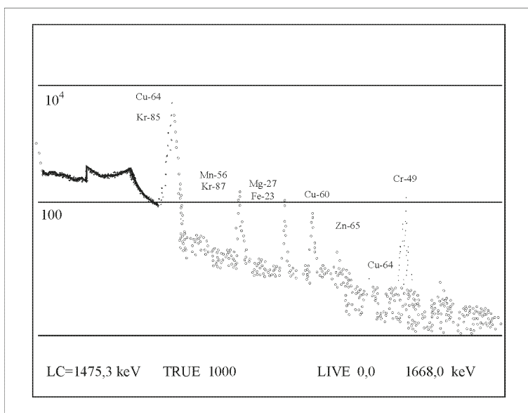
Fig. 11(a). Diagram of the GFS activation analysis immediately after radiation effects
