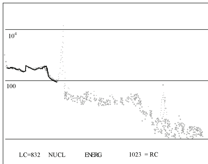
Fig. 11(b). Diagram of the GFSA activation analysis six hours after radiation effects spectrometer, respectively. Identified radioactive isotopes are recorded close to the expected energy peaks. The activity of these isotopes consists of both \gamma and \beta component. Due to the induced radioactivity, the gas ionization is intensified and the statistical time of a pulse breakdown voltage is reduced. Neutron radiation effects improve the pulse shape characteristic for a short period of time. This effect of neutron radiation disappears quickly, as the half-life time of induced activity varies from several minutes to several hours. This fact is confirmed clearly in the diagram for the activation analysis of radiated GFSA taken after six hours (Fig. 11(b)). From these diagrams one notices, that neutron activation products have completely decayed and the device GFSA had recovered back to the unirradiated state.
